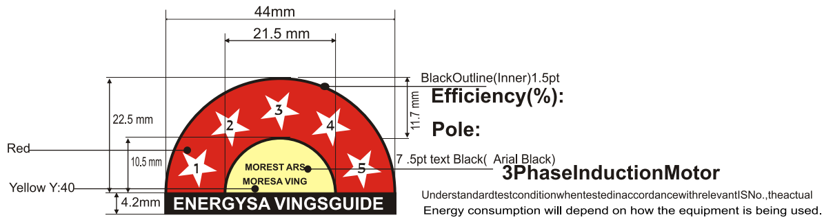
Figure1:DesignSchemeofLabel(Sample)
